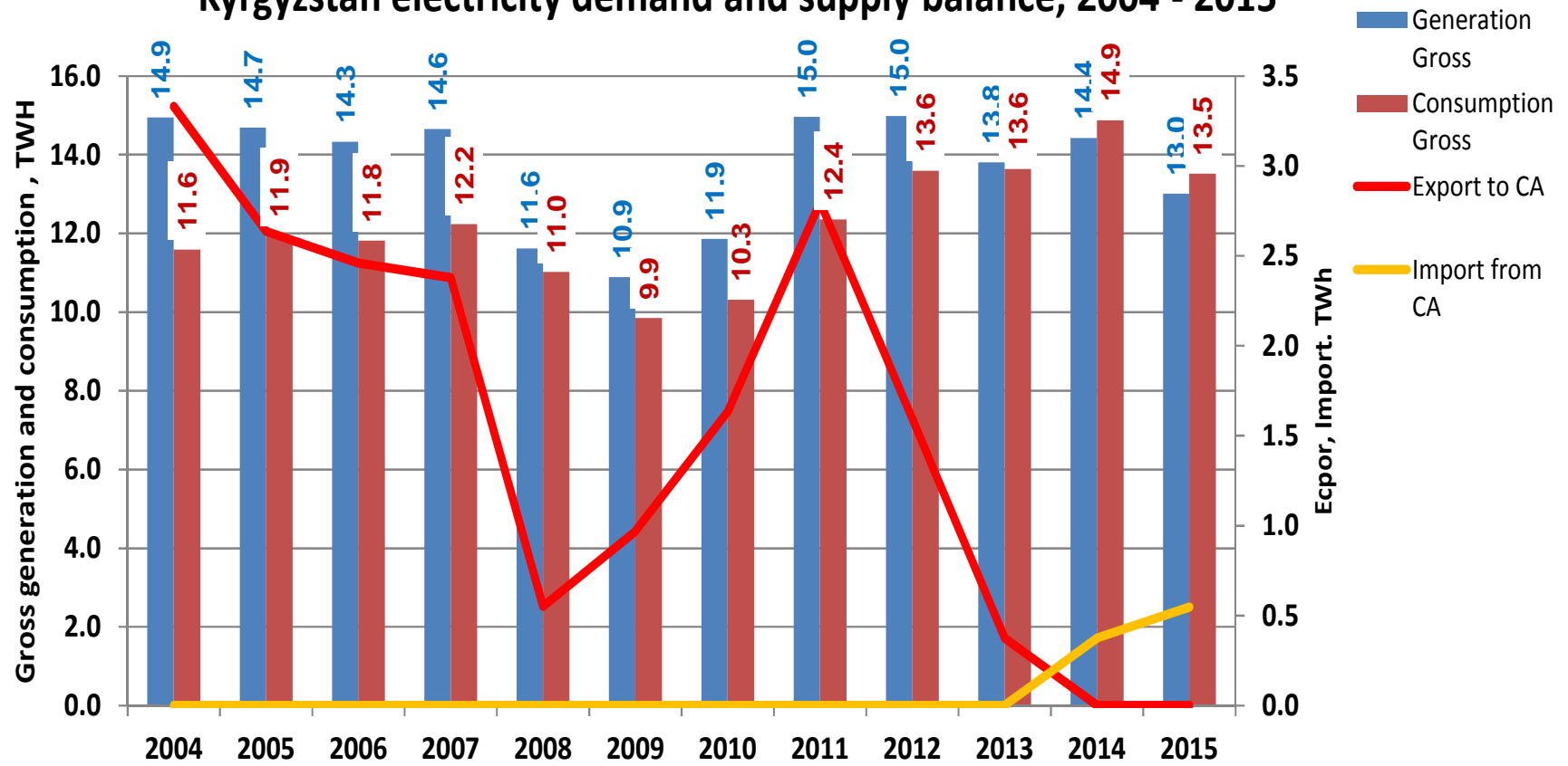
Kyrgyzstan electricity demand and supply balance, 2004 - 2015
