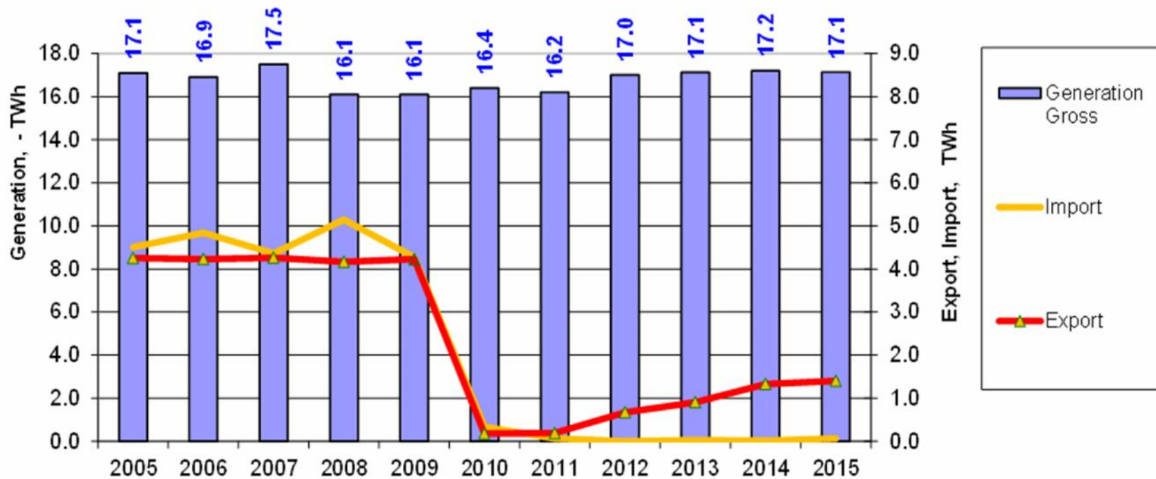
Tajikistan power system Supply and Demand balance and export / import trends with neighboring countries, 2005 - 2015
