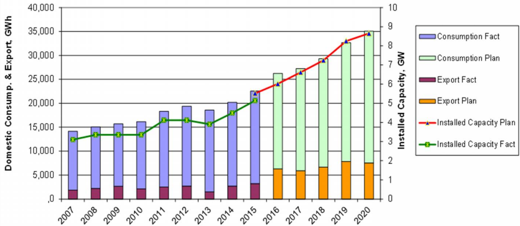
Annual Electricity Generation and export of Turkmenistan Actual 2007 - 2015 and Energy Development Concept
